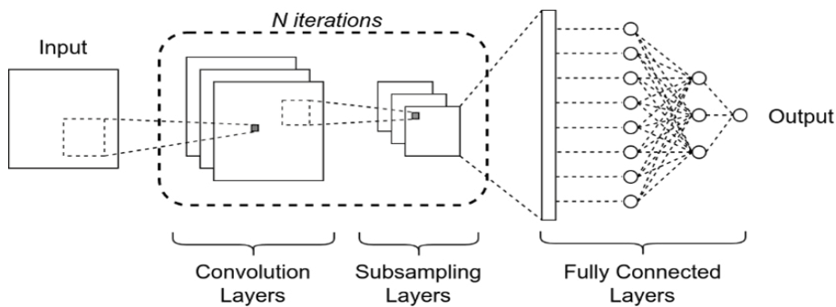
Figure 1. Basic configuration in a CNN
