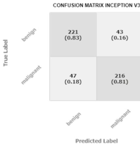
Figure 8. Confusion matrix for Inception V3
