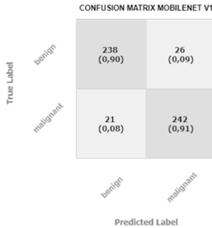
Figure 7. Confusion matrix for MobileNet V1
